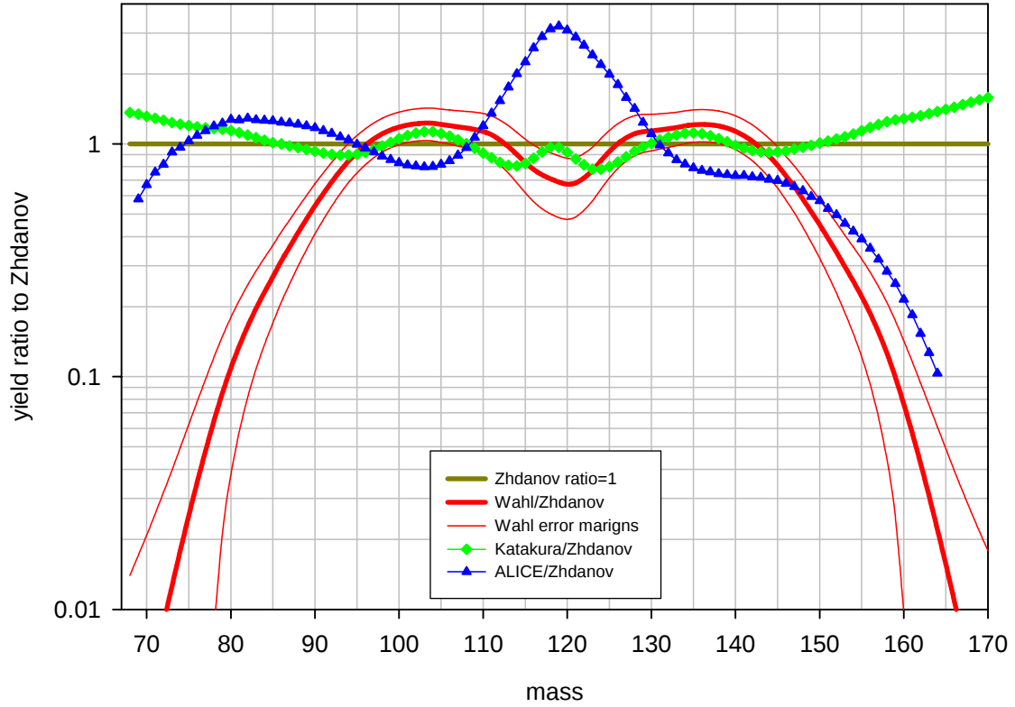
Benchmark B: ^{241}\text{Am} at 13 MeV, post neutron emission yield ratio to Zhdanov's data
